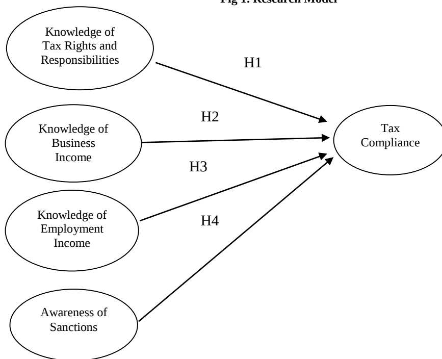
Fig 1. Research Model
