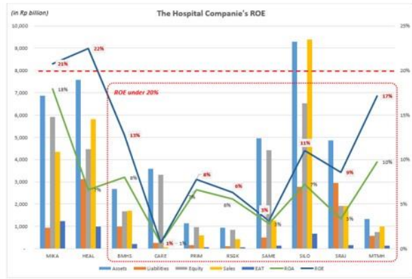
Figure 8 Variables Correlation
