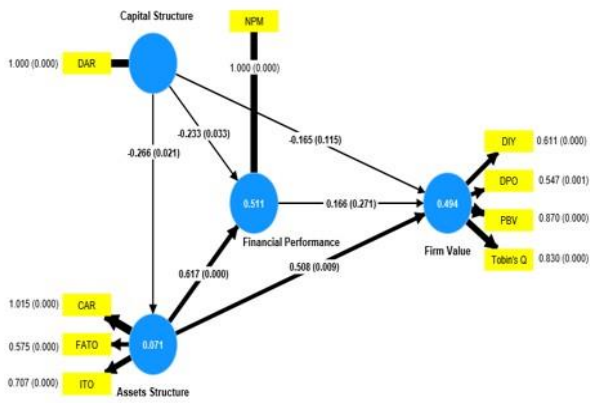
Figure 8 Variables Correlation
